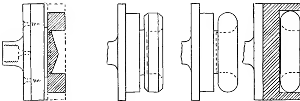
FIG. 327. TURNING A RING—THIRD METHOD.
